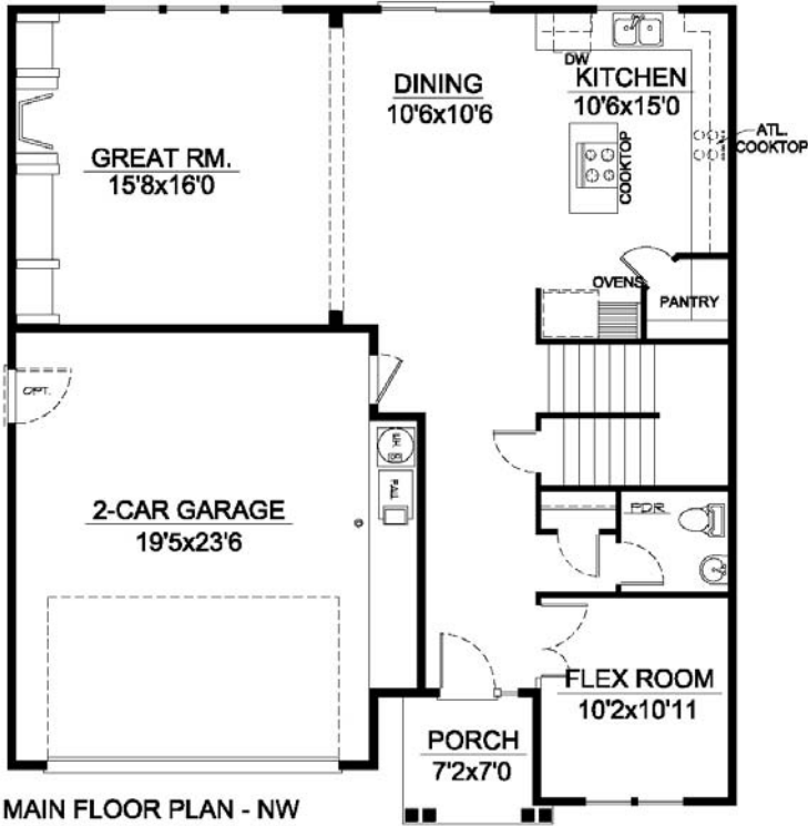
MAIN FLOOR PLAN - NW
