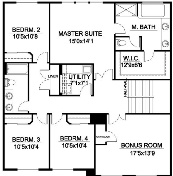
UPPER FLOOR PLAN - NW
